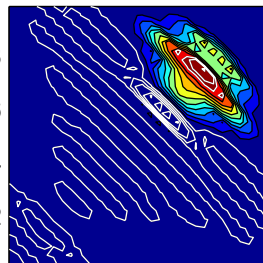
Superbee (no multi-dim)
