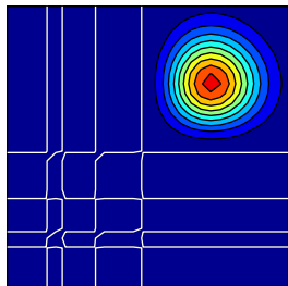
Superbee flux limiter
