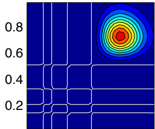
2nd order centered
