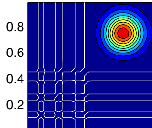
4th order centered
