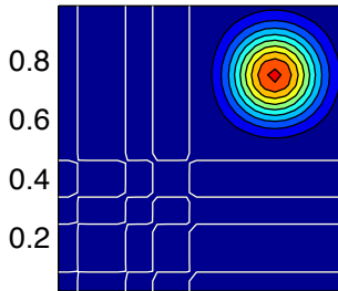
3rd order upwind
