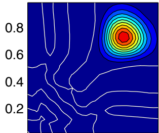
0.2 0.4 0.6 0.8 Lax-Wendroff
