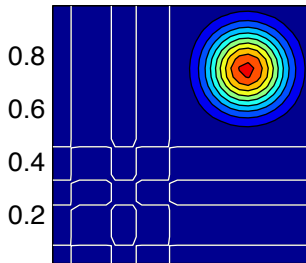
0.2 0.4 0.6 0.8 3-DST Sweby \mu=\mu(c)
