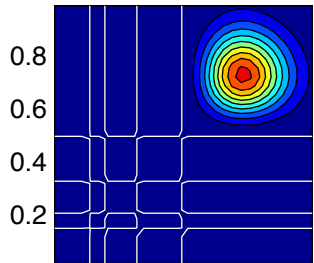
0.2 0.4 0.6 0.8 Superbee flux limiter
