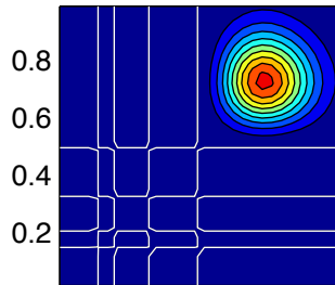
0.2 0.4 0.6 0.8 Superbee (no multi-dim)
