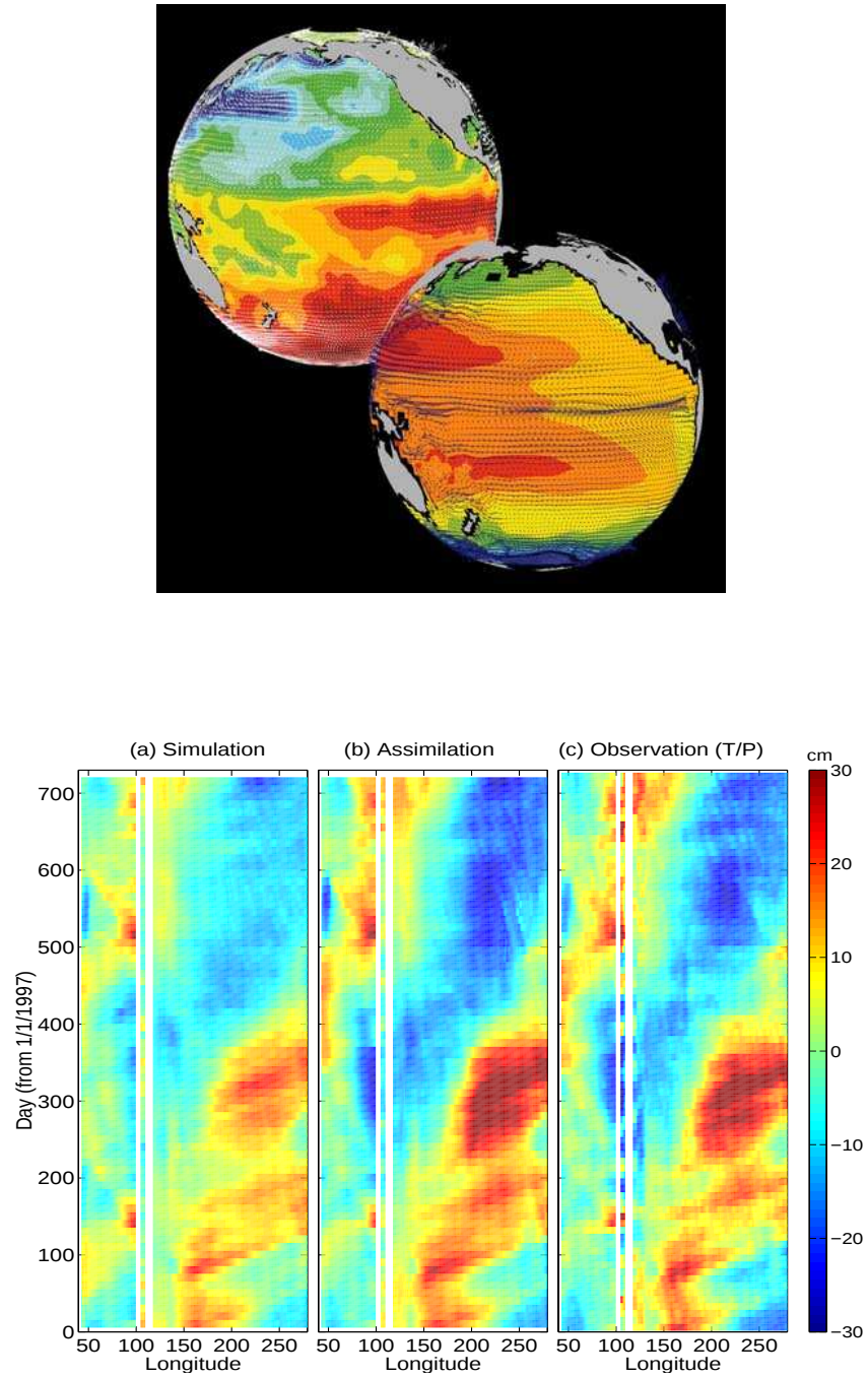
Figure 1.11: Top panel shows circulation patterns from a multi-year, global circulation simulation constrained by Topex altimeter data and WOCE cruise observations. Bottom panel shows the equatorial sea-surface height in unconstrained (left), constrained (middle) simulations and in observations. This output is from a higher resolution, shorter duration experiment with equatorially enhanced grid spacing.
