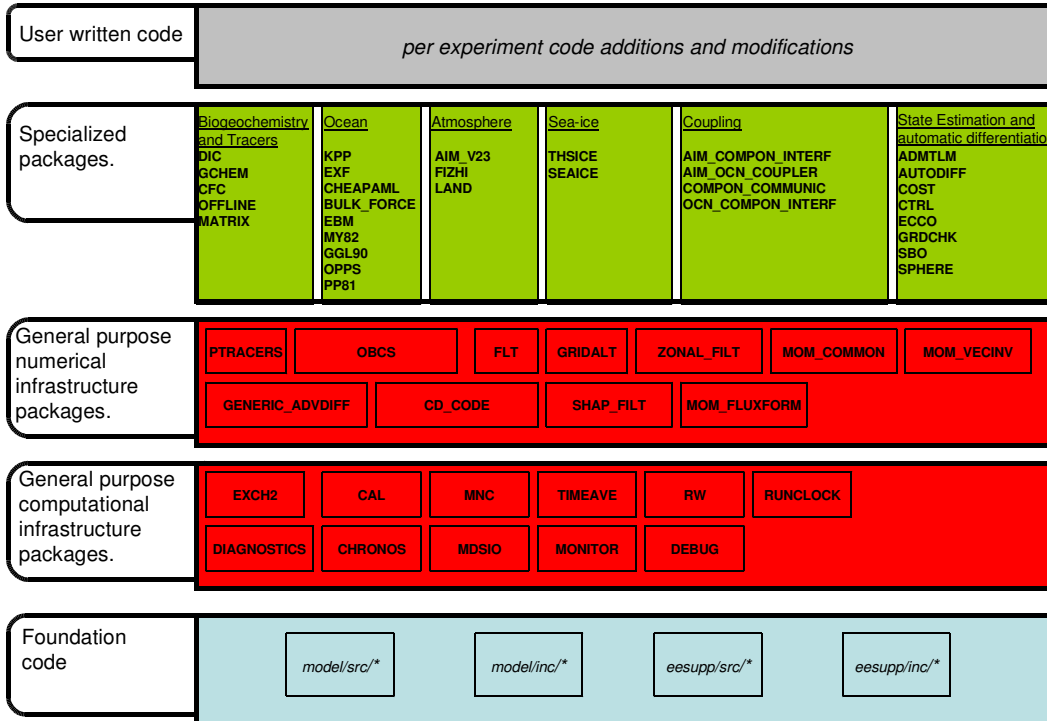
Figure 6.1: Hierarchy of code layers that are assembled to make up an MITgcm simulation. Conceptually (and in terms of code organization) MITgcm consists of several layers. At the base is a layer of core software that provides a basic numerical and computational foundation for MITgcm simulations. This layer is shown marked Foundation Code at the bottom of the figure and corresponds to code in the italicised subdirectories on the figure. This layer is not organized into packages. All code above the foundation layer is organized as packages. Much of the code in MITgcm is contained in packages which serve as a useful way of organizing and layering the different levels of functionality that make up the full MITgcm software distribution. The figure shows the different packages in MITgcm as boxes containing bold face upper case names. Directly above the foundation layer are two layers of general purpose infrastructure software that consist of computational and numerical packages. These general purpose packages can be applied to both online and offline simulations and are used in many different physical simulation types. Above these layers are more specialized packages.
