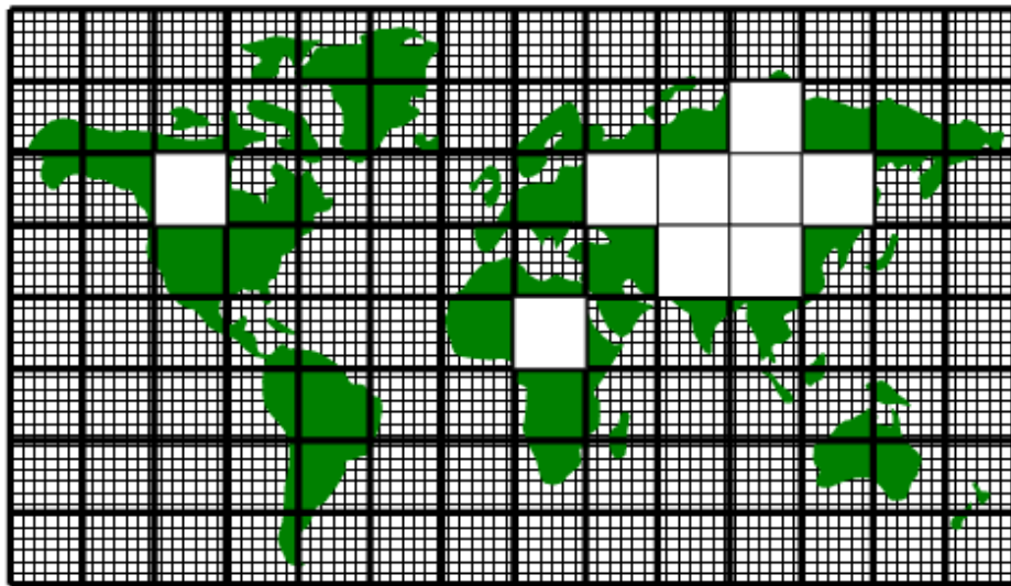
Figure 4.4: A global grid subdivided into tiles. Tiles contain an interior region and an overlap region. Overlap regions are periodically updated from neighboring tiles.
