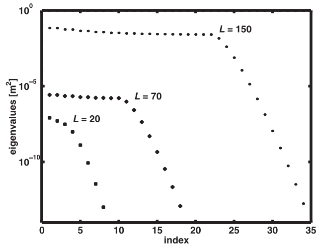
Figure 5. Eigenvalue spectrum of the geoid error covariance matrix for the three cases L = 20 , L = 70 , and L = 150 .
