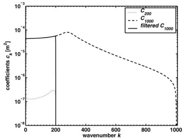
Figure 4. Fourier spectra of geoid height error covariance functions: commission error up to L = 200 ( C_{200} ), commission plus omission error ( C_{1000} ), and a filtered version of the latter with cut-off k = 200 .
