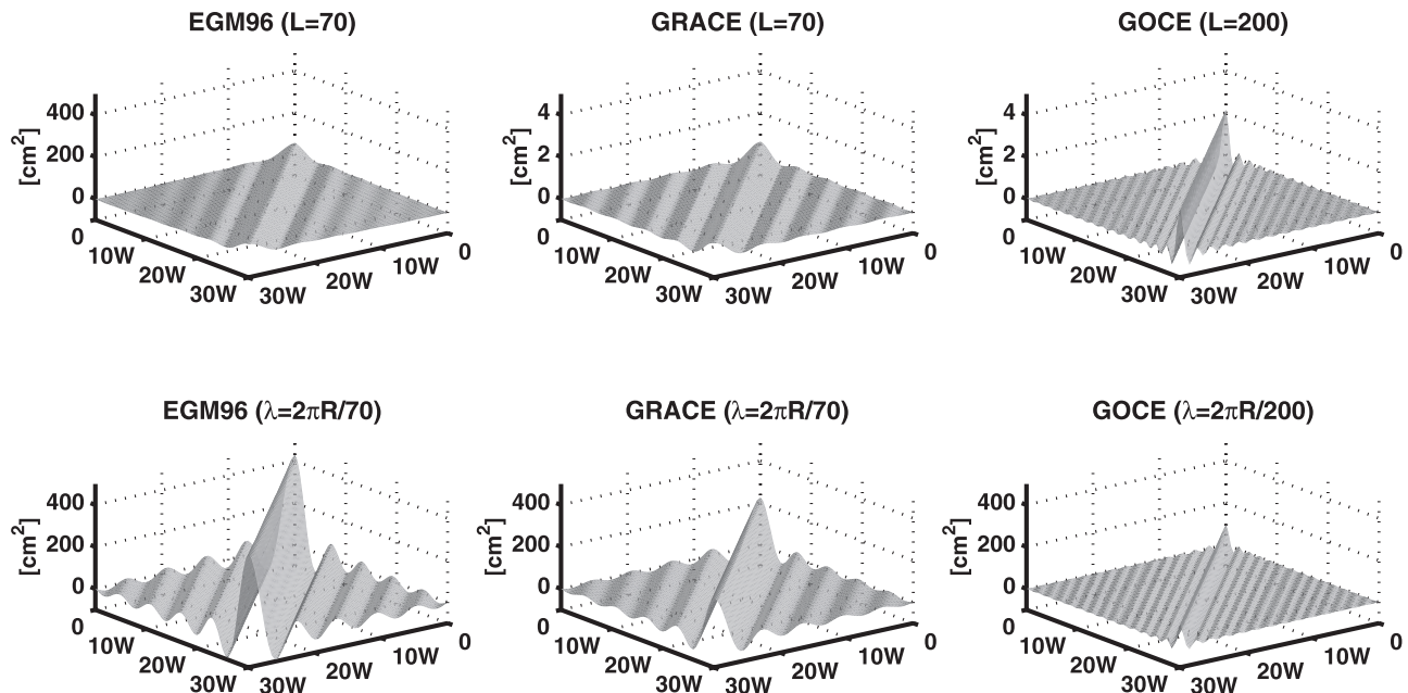
Figure 8. SSH error covariance matrices \mathbf{R}_c (top) without omission error (note the different scale for GRACE and GOCE) and (bottom) with omission error after filtering out all small scales according to the maximum degree and order used for EGM96, GRACE, and GOCE, for the zonal sample section of section 3.
