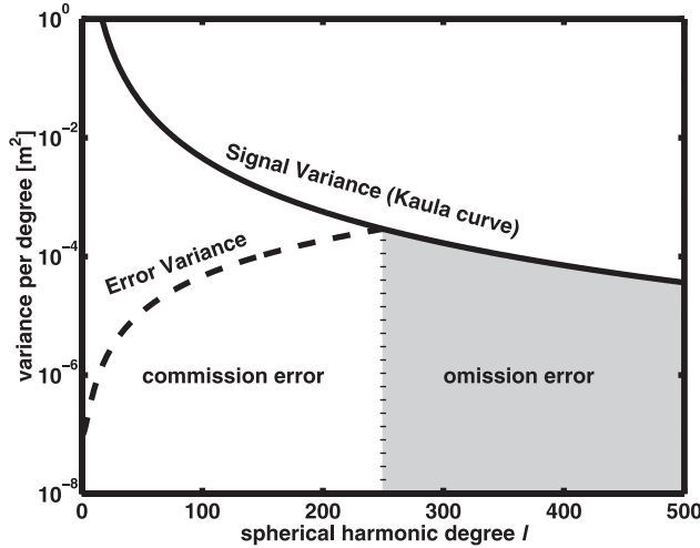
Figure 2. Schematic plot of signal variance per degree using Kaula's law and a synthetic error spectrum.
