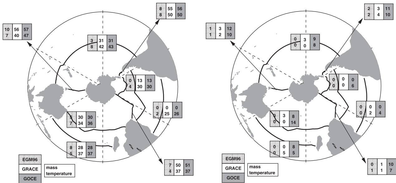
Figure 9. Error reduction relative to hydrography alone solution (left) without omission error (NOM) and (right) with omission error (FOM). The upper numbers are the error reductions of mass transports (in %), the lower numbers those of temperature transports.
